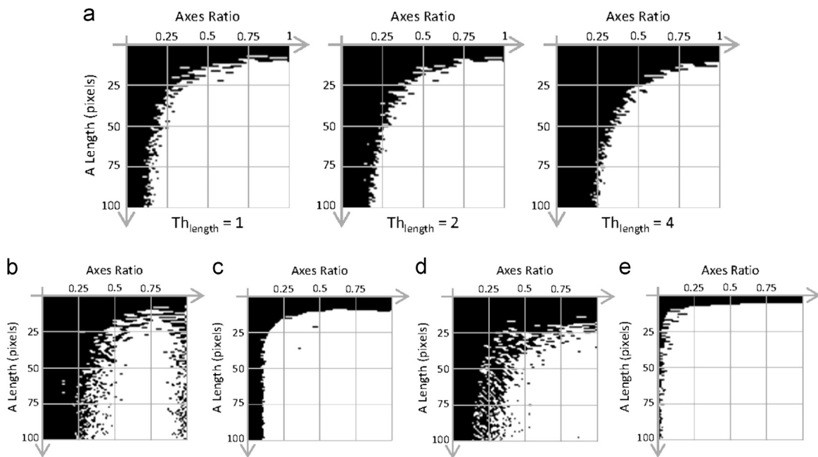
Fig. 16. Working conditions, with respect to major semi-axis length (vertical axis, from 1 to 100) and axes ratio B/A (horizontal axis, from 0 to 1). (a) Ours, varying Th_{length} , (b) Zhang and Liu [16], (c) Basca et al. [14], (d) Libuda et al. [22], and (e) Prasad et al. [25].
