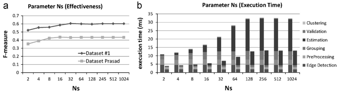
Fig. 14. Effectiveness and execution time varying N_s . (a) F -measure. (b) Execution time on Dataset #1 (left column) and Dataset Prasad (right column).
