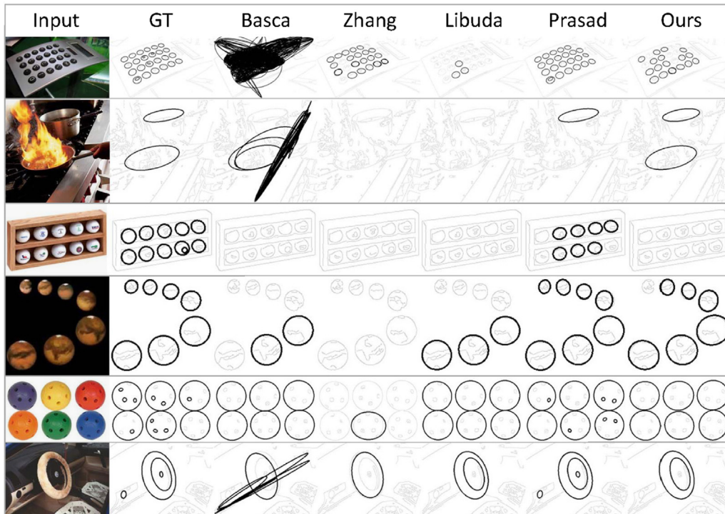
Fig. 24. Results on Dataset Prasad.
