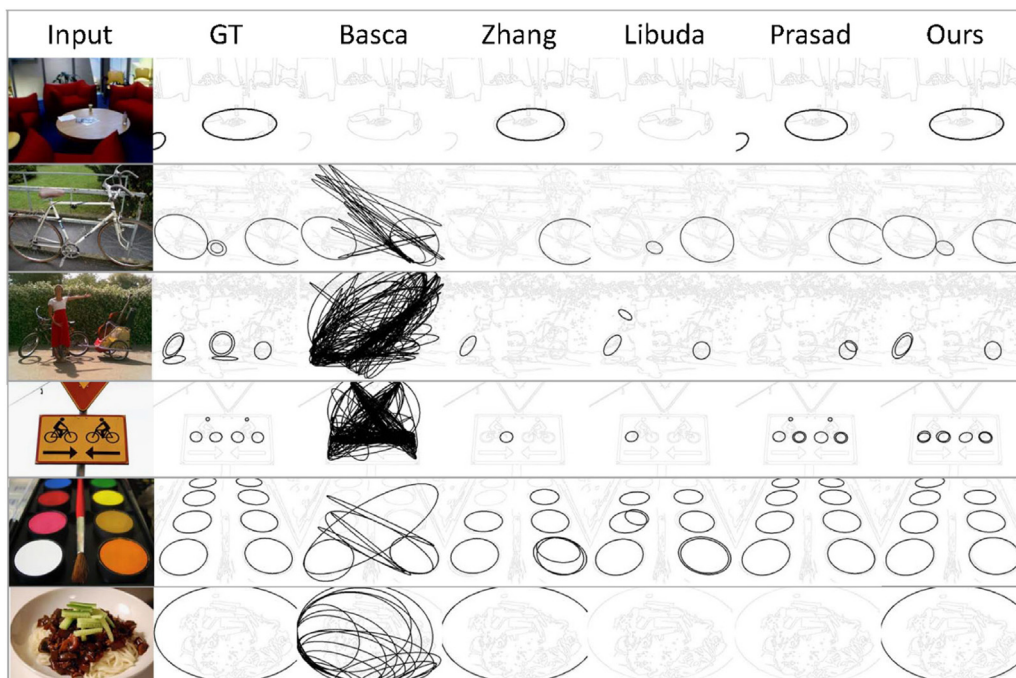
Fig. 25. Results on Dataset #1.
