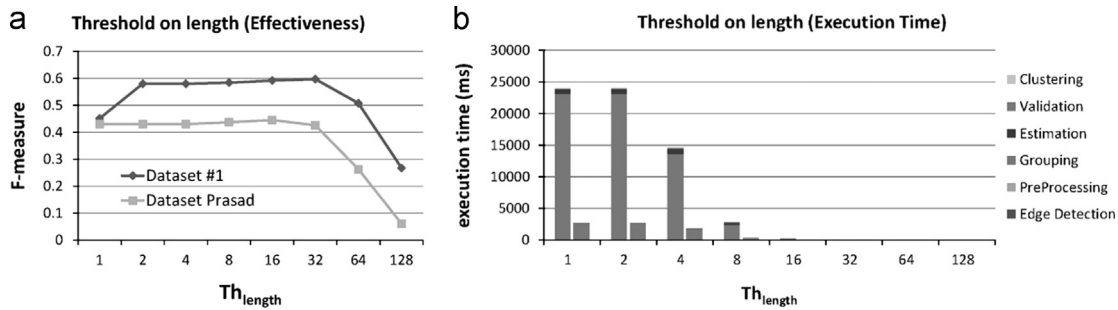
Fig. 10. Performance varying Th_{length} . (a) F-measure. (b) Execution time on Dataset #1 (left column) and Dataset Prasad (right column).
