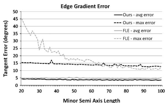
Fig. 9. The maximum and average error of our method and Fast Line Extraction [39].
