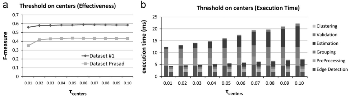
Fig. 13. Performance varying \tau_{centers} , where (Th_{centers} = \tau_{centers} \times \text{image diagonal}) . (a) F -measure. (b) Execution time on Dataset #1 (left column) and Dataset Prasad (right column).
