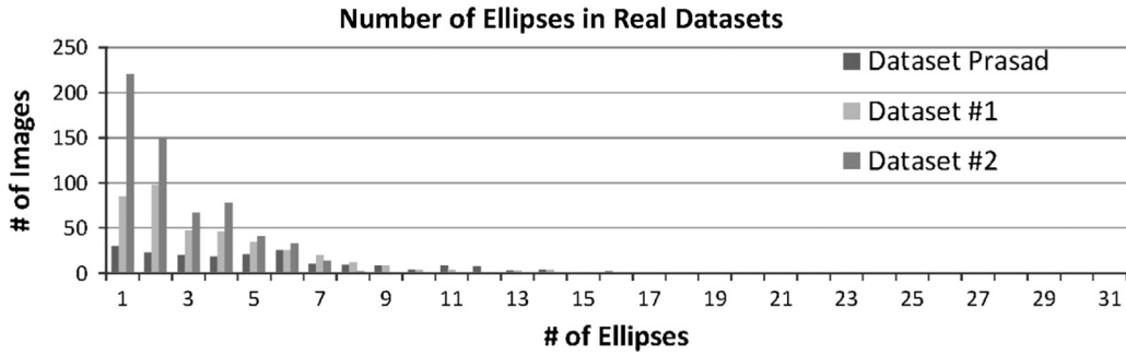
Fig. 20. Images per number of ellipses in real datasets.
