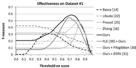
Fig. 22. Graph reporting the F -measure varying Th_\sigma on Dataset #1.
