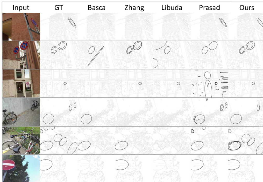
Fig. 26. Results on Dataset #2.
