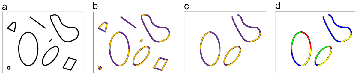
Fig. 4. Toy example of arc detection. Best viewed in colors. (a) Edge points. (b) Direction classification. (c) Removal of short and straight arcs. (d) Quadrants classification. (For interpretation of the references to color in this figure caption, the reader is referred to the web version of this paper.)
