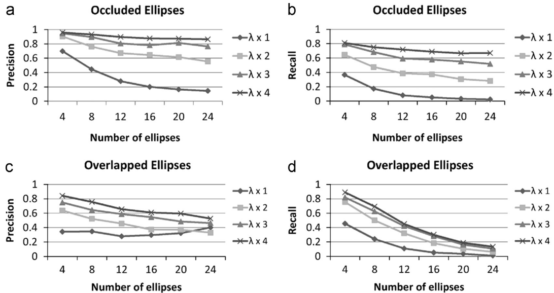
Fig. 18. Evaluation on Dataset Chia [24] of the proposed method increasing the value of \lambda . (a) Precision. (b) Recall. (c) Precision. (d) Recall.
