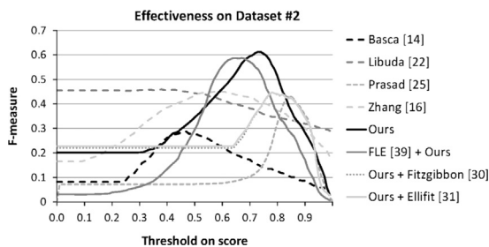
Fig. 23. Graph reporting the F -measure varying Th_\sigma on Dataset #2.
