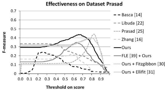
Fig. 21. Graph reporting the F -measure varying Th_\sigma on Dataset Prasad.
