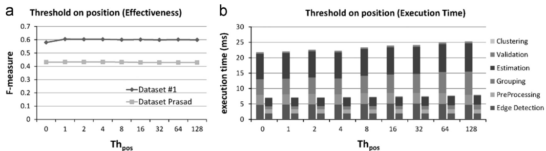
Fig. 12. Performance varying Th_{pos} . (a) F-measure. (b) Execution time on Dataset #1 (left column) and Dataset Prasad (right column).
