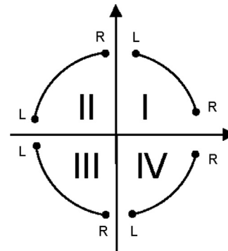
Fig. 5. Mutual position.
