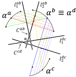
Fig. 8. Estimated center of the ellipse.
