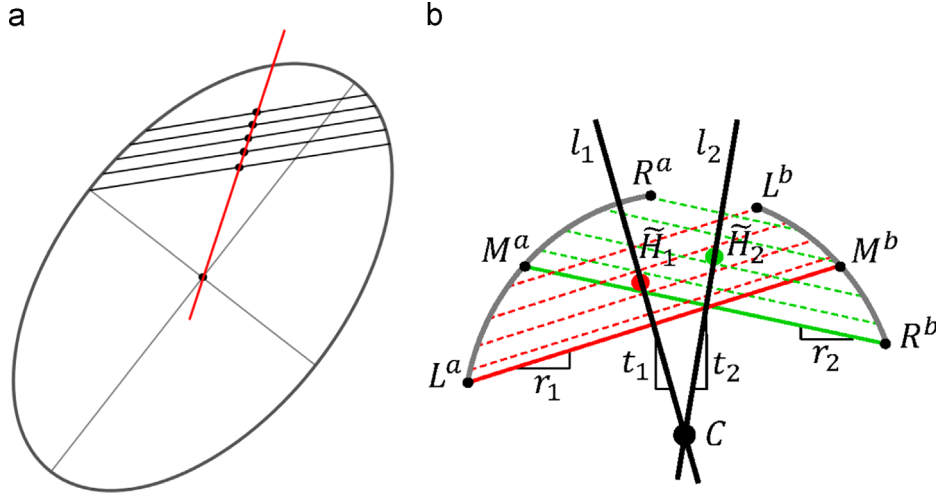
Fig. 6. Method for estimating the ellipse center. (a) The midpoints of a set of parallel chords and its center are collinear, (b) Geometric features to compute the center.
