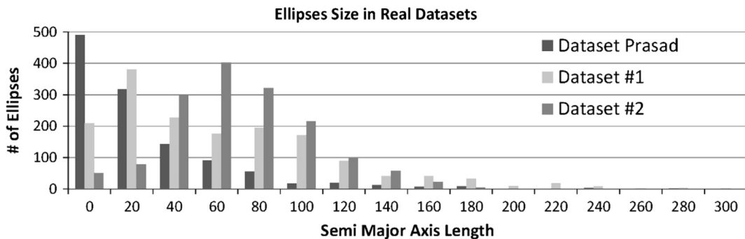
Fig. 19. Number of ellipses per length of the major semi-axes in real datasets.
