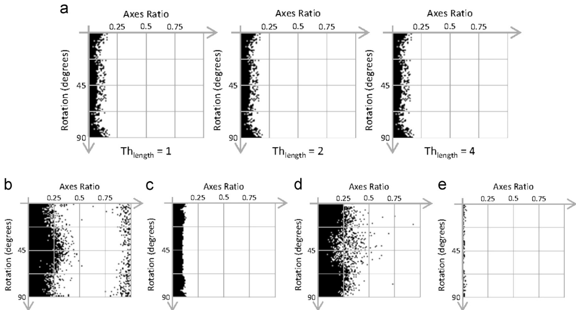
Fig. 15. Working conditions, with respect to rotation (vertical axis, from 0° to 90°) and axes ratio B/A (horizontal axis, from 0 to 1). (a) Ours, varying Th_{length} , (b) Zhang and Liu [16], (c) Basca et al. [14], (d) Libuda et al. [22], and (e) Prasad et al. [25].
