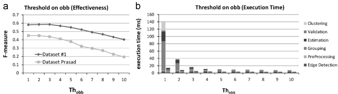
Fig. 11. Performance varying Th_{obb} . (a) F-measure. (b) Execution time on Dataset #1 (left column) and Dataset Prasad (right column).
