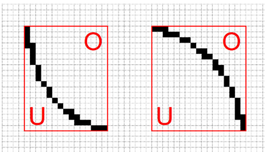
Fig. 3. Convexity classification.
